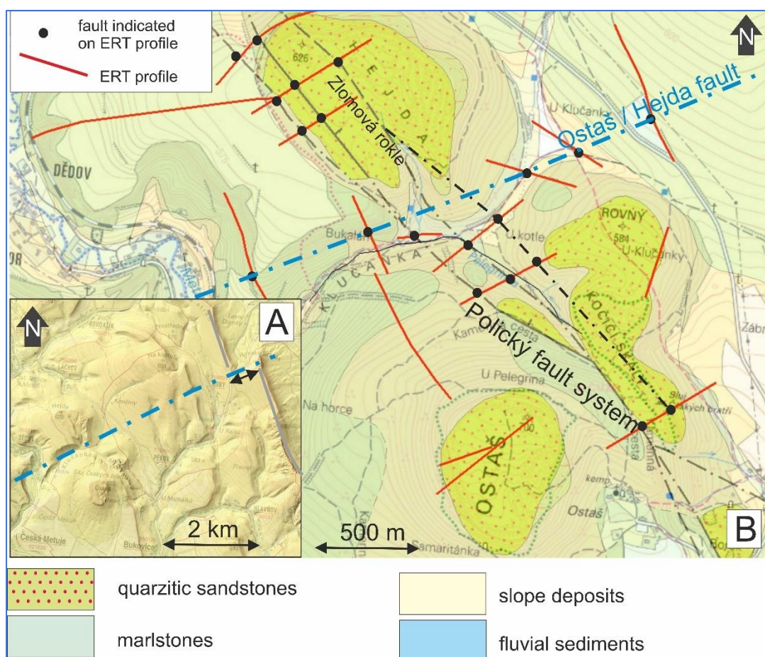
Fig. 1. A – Map (strictly DTM) illustrating the sidestep of the Broumovské stěny kuesta front line at the Ostaš/Hejda fault line. B – Topographical and geological situation of fault systems and ERT profiles (2015-2021) in the study area.
